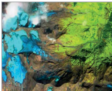
Sentinel-2 image (band combination 11, 8a, 2), Fuschertal valley, at mapping season (August) revealing: vegetation (green), rocks (brown), glacier (dark blue), snow (light blue), clouds (white).
