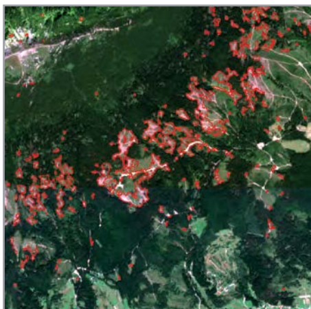
Forest clear cuts detected between 2015 and 2017 using Sentinel-2 data over the mountain forest in the Nowy Targ District, Poland.
